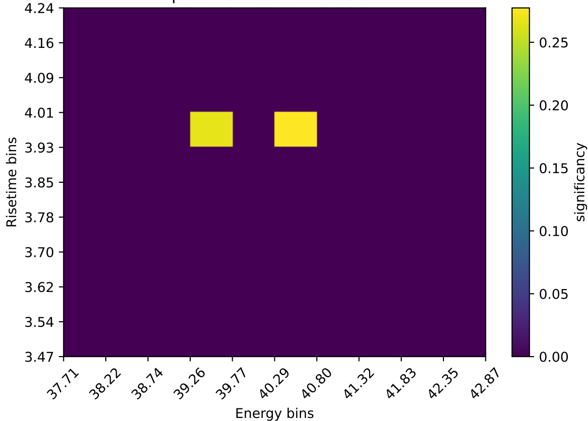
pion distribution 40.0GeV
